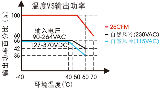
LOF450-20B24/27/36/48/54 (满载 450W 带 25CFM 风扇)
