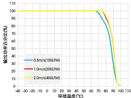
VCB4805EBO-100WFR3温度降额曲线
